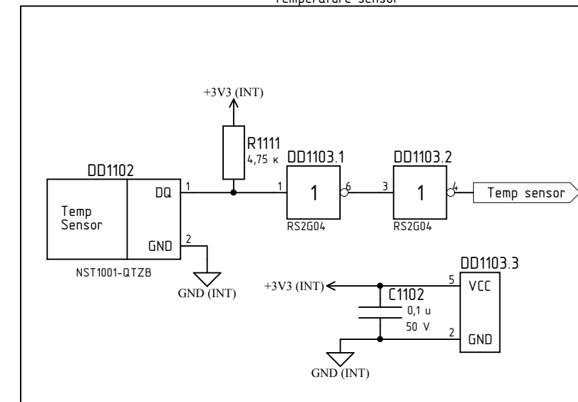
Temperature sensor
